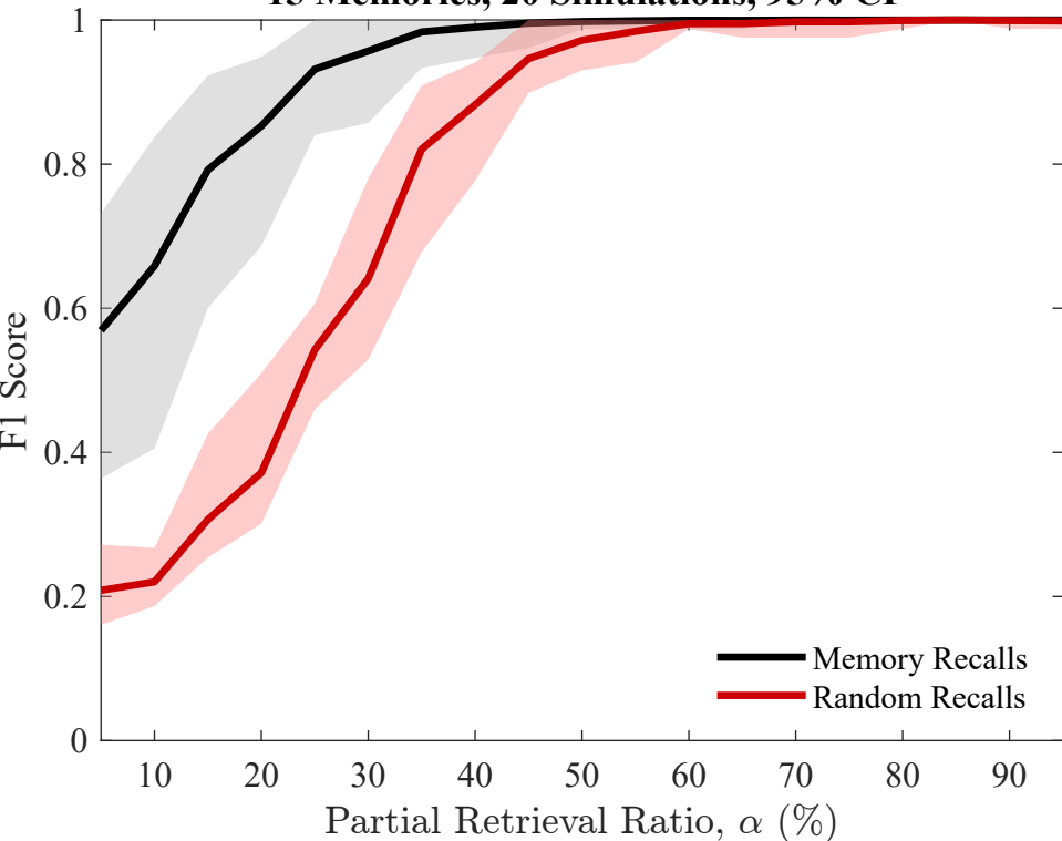
F1 Score Performance — SVM Classification 15 Memories, 20 Simulations, 95% CI
