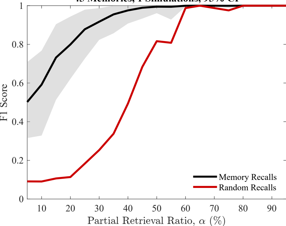
F1 Score Performance — SVM Classification 45 Memories, 1 Simulations, 95% CI
