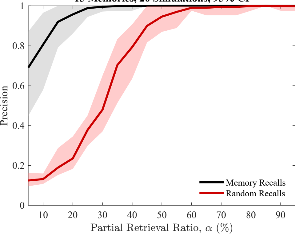
Precision Performance — SVM Classification 15 Memories, 20 Simulations, 95% CI
