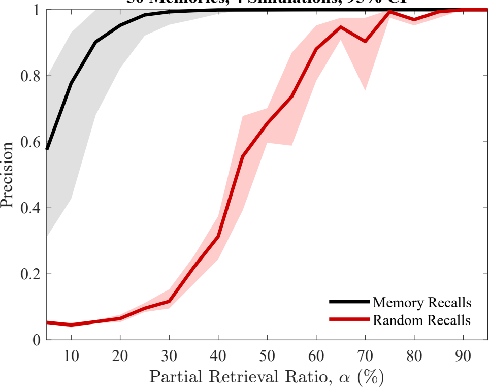
Precision Performance — SVM Classification 50 Memories, 4 Simulations, 95% CI
