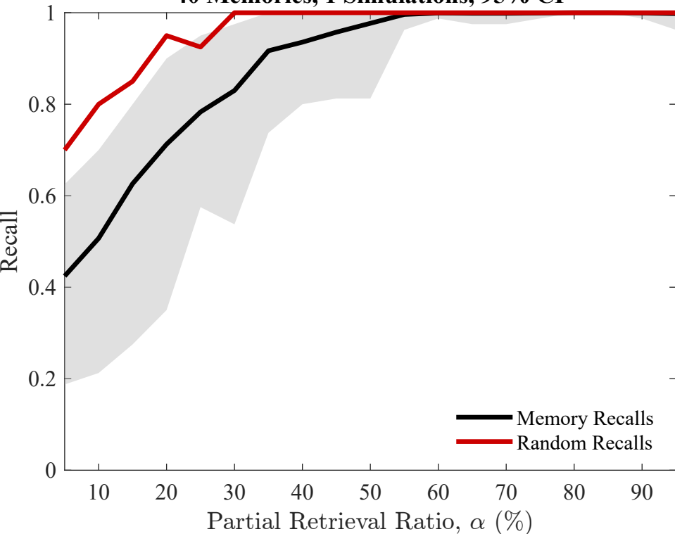
Recall Performance — SVM Classification 40 Memories, 1 Simulations, 95% CI
