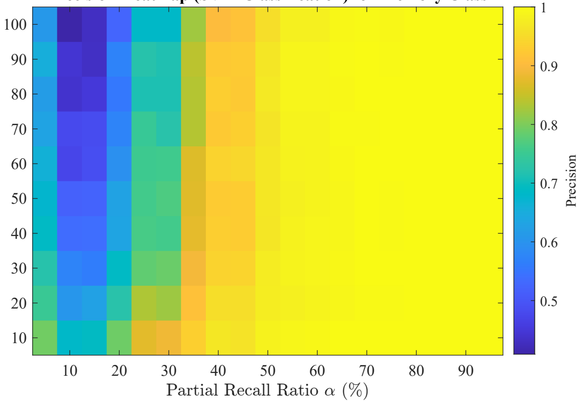
Precision Heatmap (SVM Classification) for Memory Class
