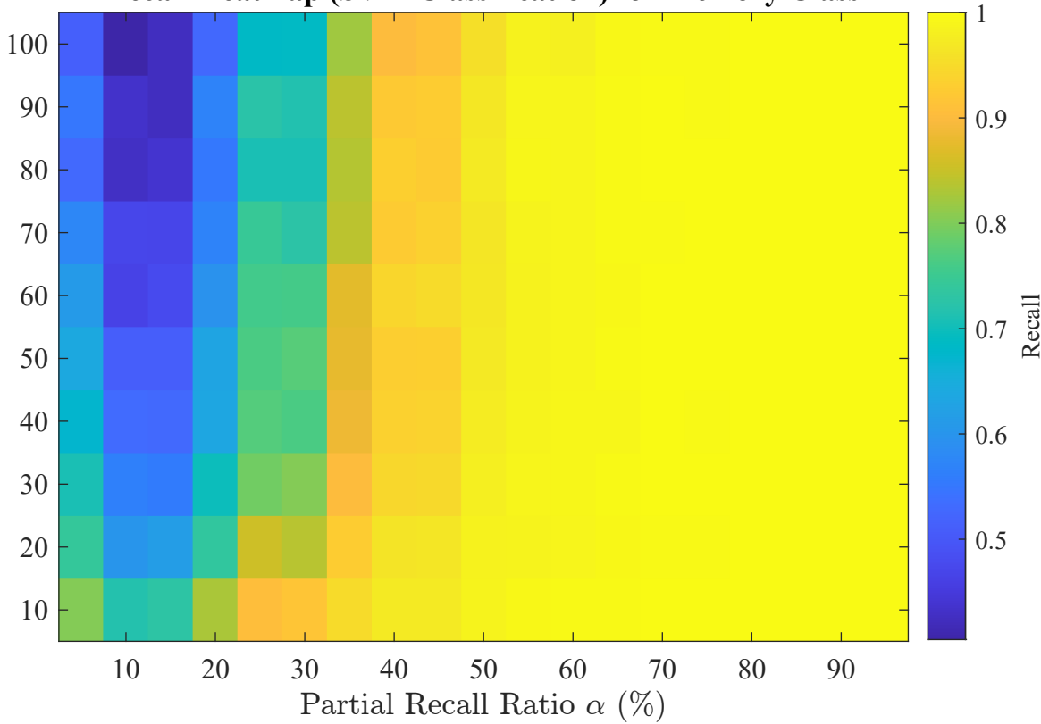
Recall Heatmap (SVM Classification) for Memory Class
