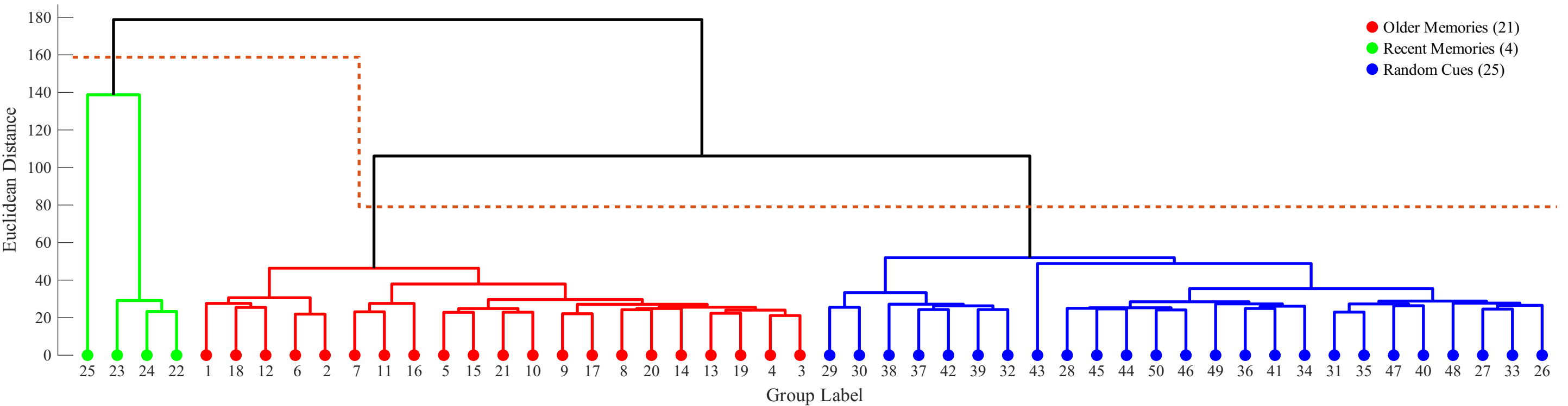
Dendrogram
