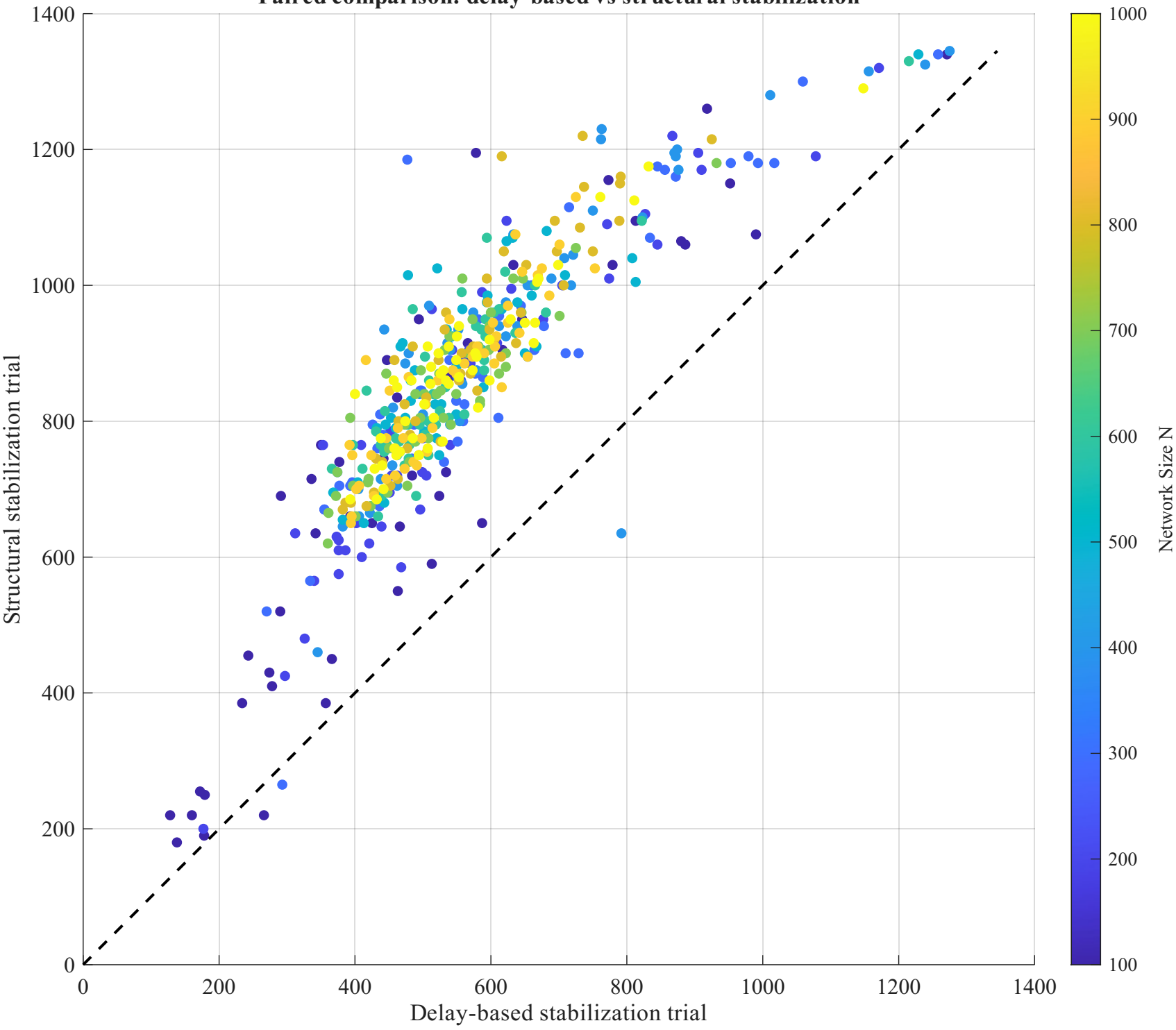
Paired comparison: delay-based vs structural stabilization
