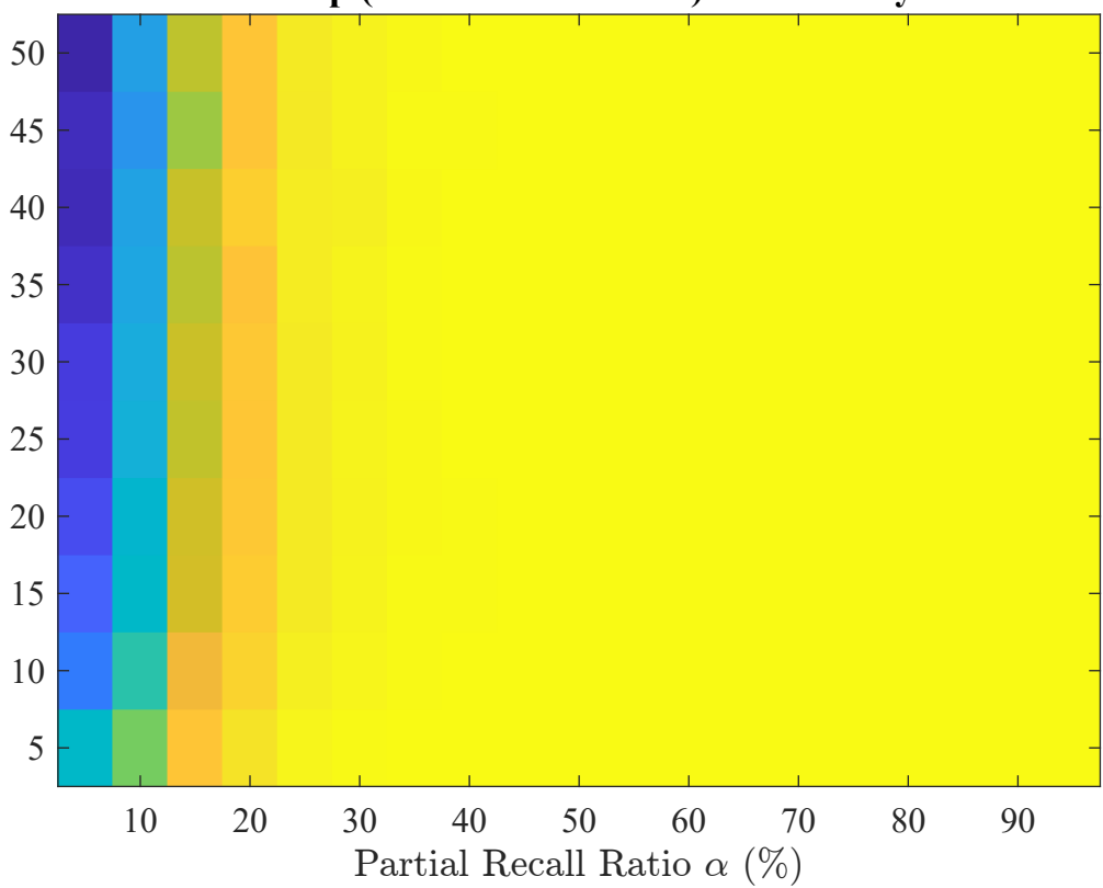
F1 Heatmap (SVM Classification) for Memory Class
