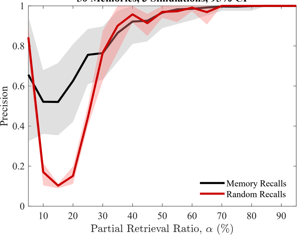
Precision Performance — SVM Classification 50 Memories, 3 Simulations, 95% CI
