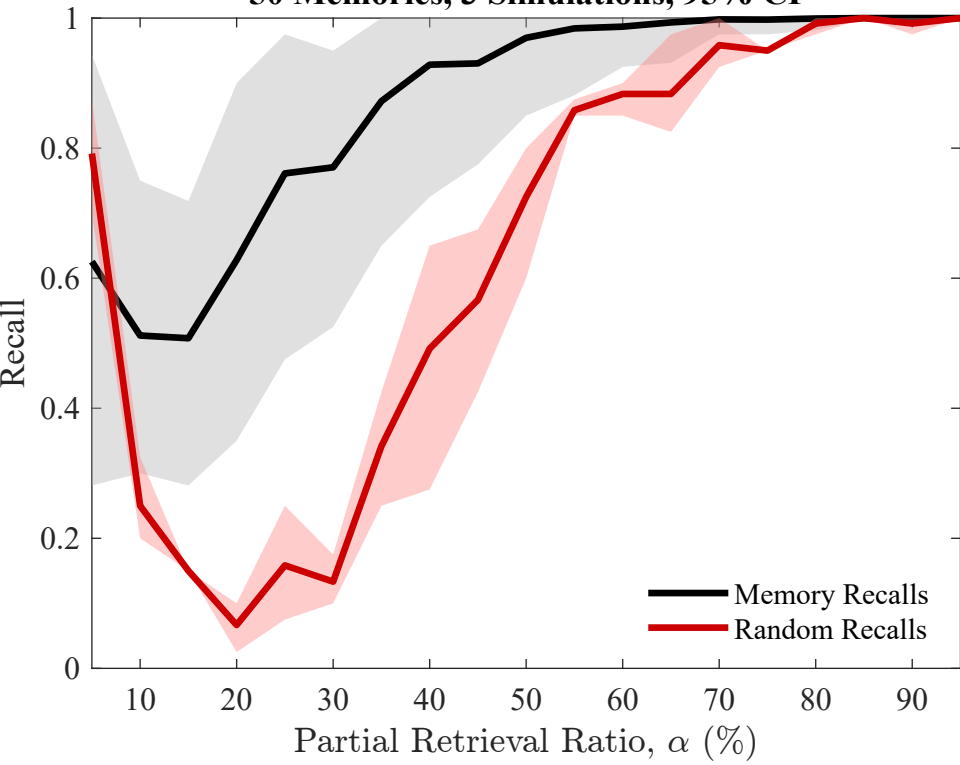
Recall Performance — SVM Classification 50 Memories, 3 Simulations, 95% CI
