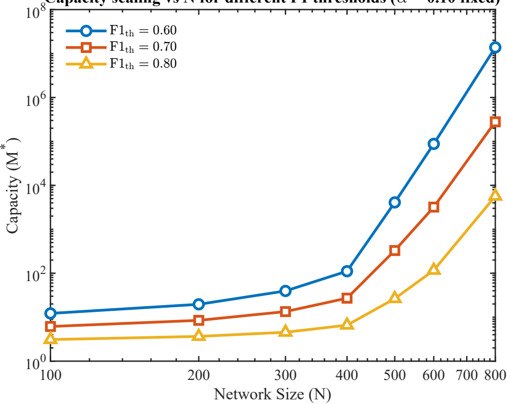
Capacity scaling vs N for different F1 thresholds ( \alpha = 0.10 fixed)
