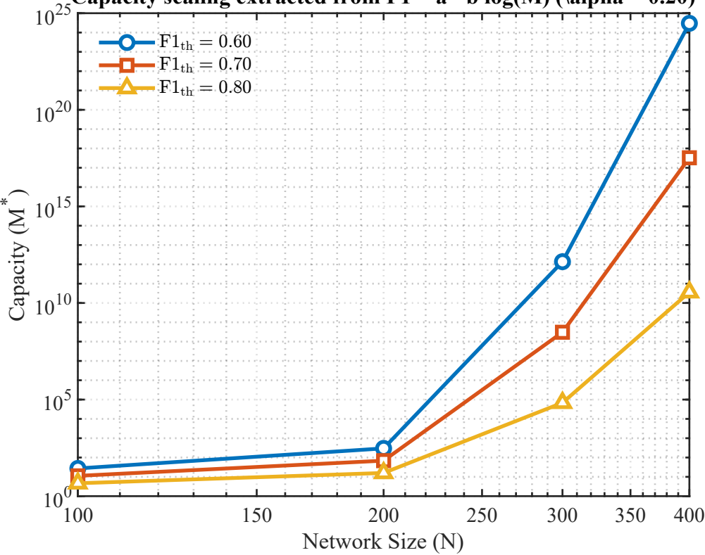
Capacity scaling extracted from F1 = a - b \log(M) ( \alpha = 0.20 )
