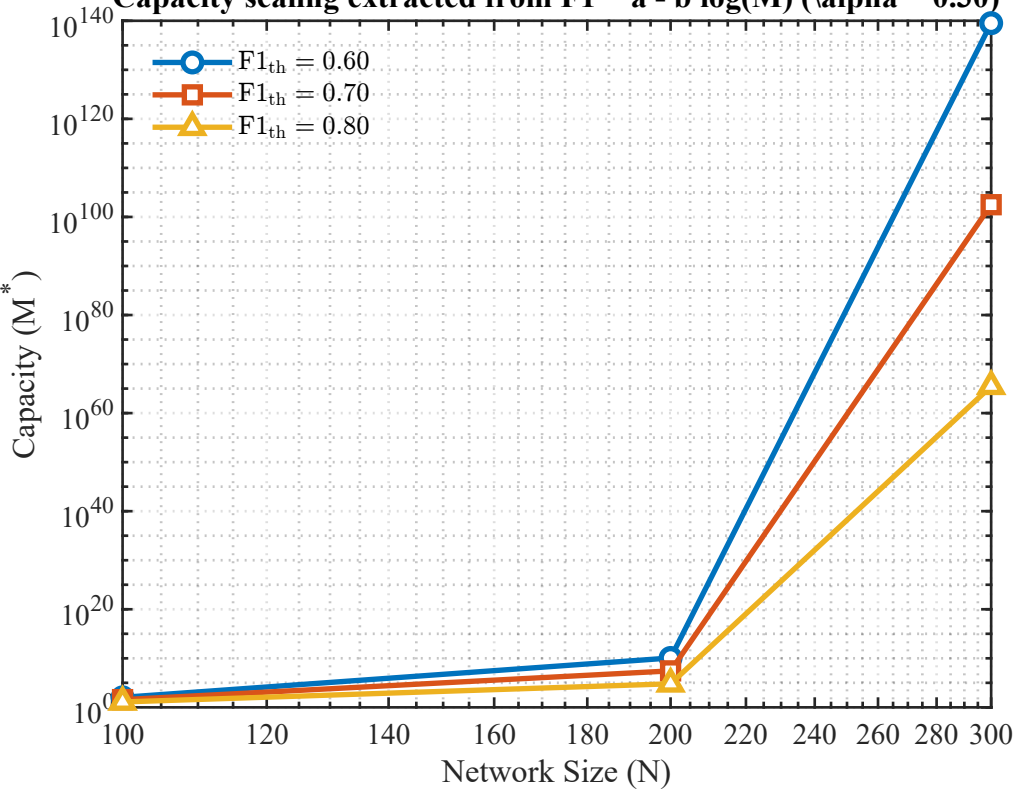
Capacity scaling extracted from F1 = a - b \log(M) ( \alpha = 0.30 )
