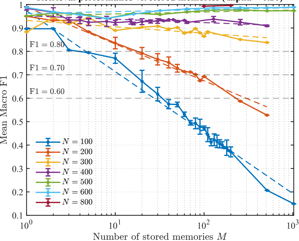
Retrieval performance vs. stored memories ( \alpha = 0.20 )
