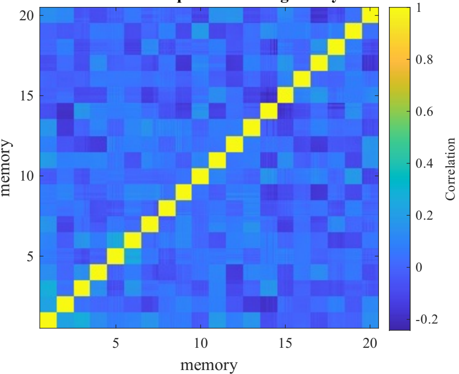
Memories Sequences Orthogonality
