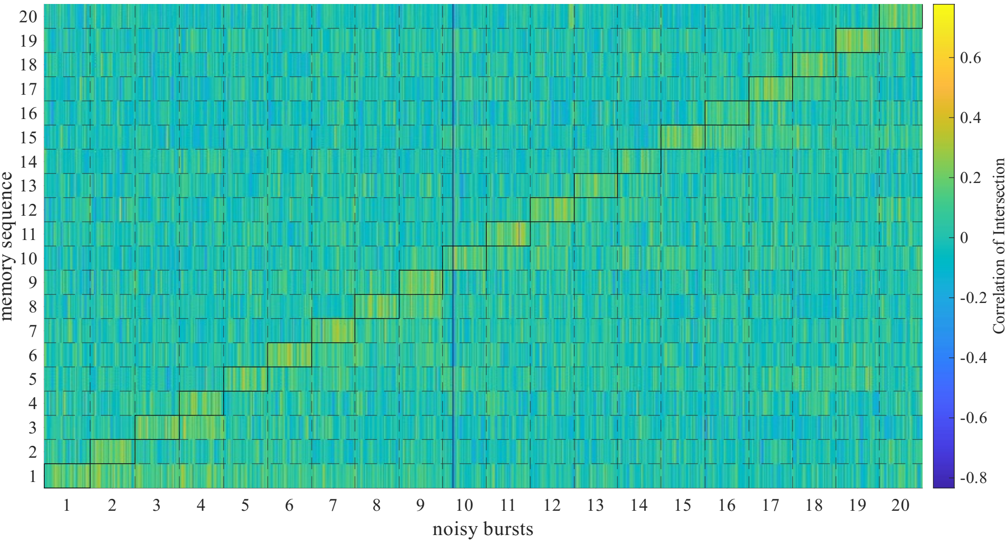
Similarity of Memories with Noisy Spontaneous Bursts
