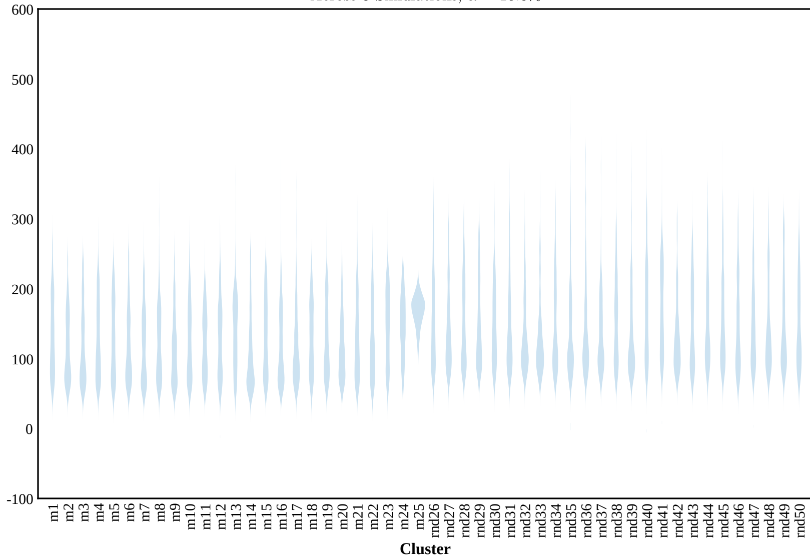
Aggregated Intra-cluster Distances Across 8 Simulations, \alpha = 10.0\%
