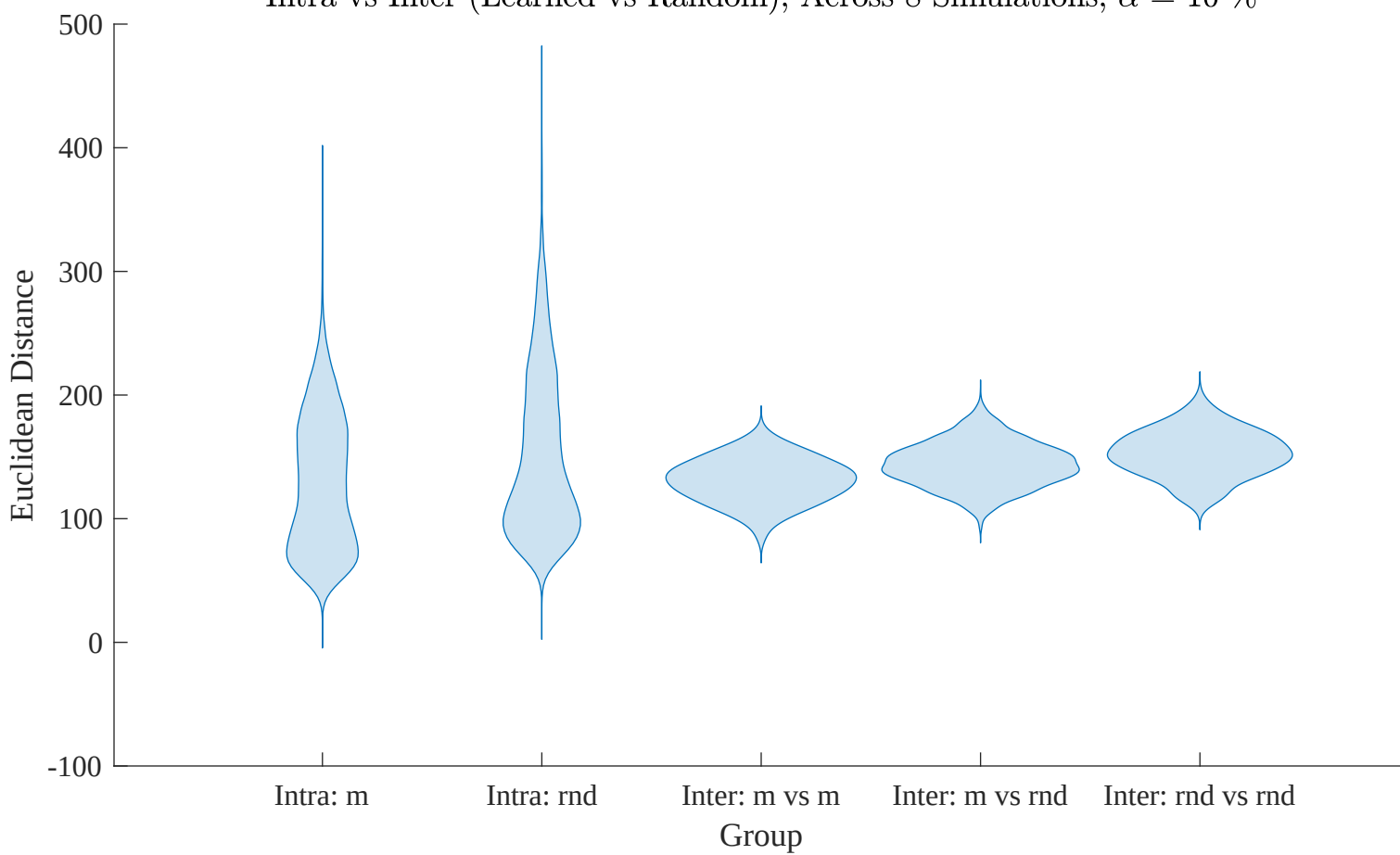
Cluster Distance Comparison Intra vs Inter (Learned vs Random), Across 8 Simulations, \alpha = 10\%
