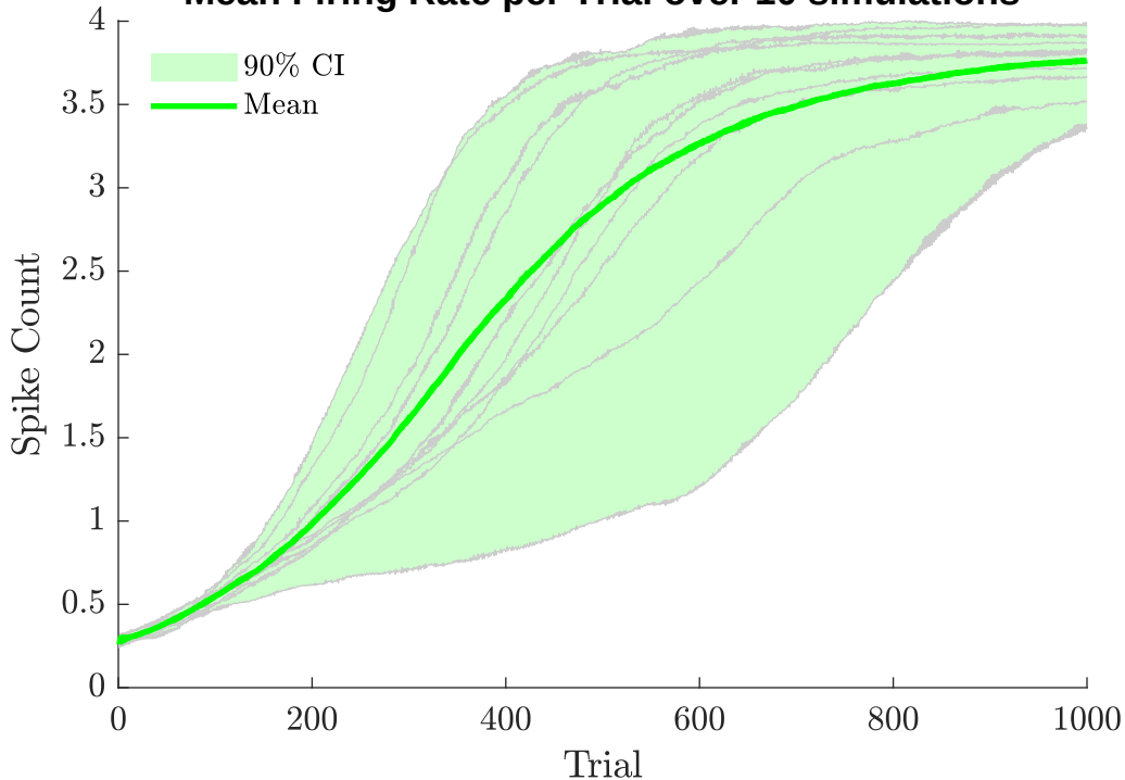
Mean Firing Rate per Trial over 10 simulations
