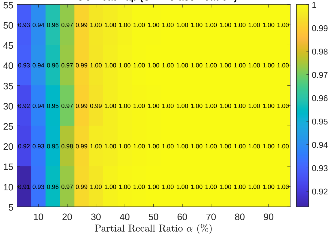
AUC Heatmap (SVM Classification)
