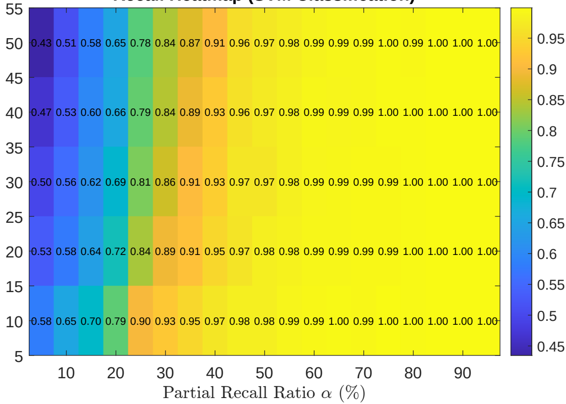
Recall Heatmap (SVM Classification)
