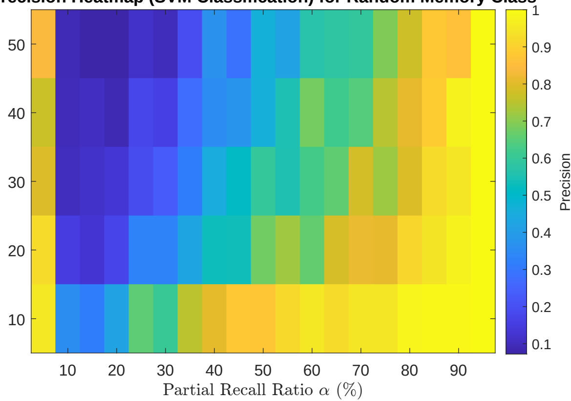
Precision Heatmap (SVM Classification) for Random Memory Class
