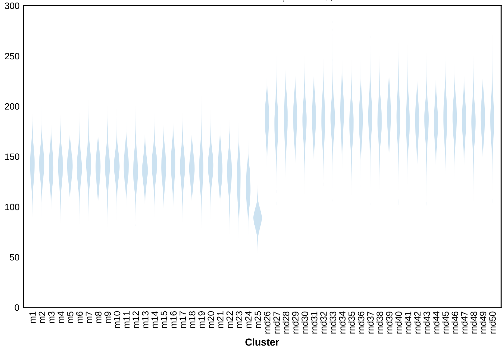
Aggregated Intra-cluster Distances Across 8 Simulations, \alpha = 50.0\%
