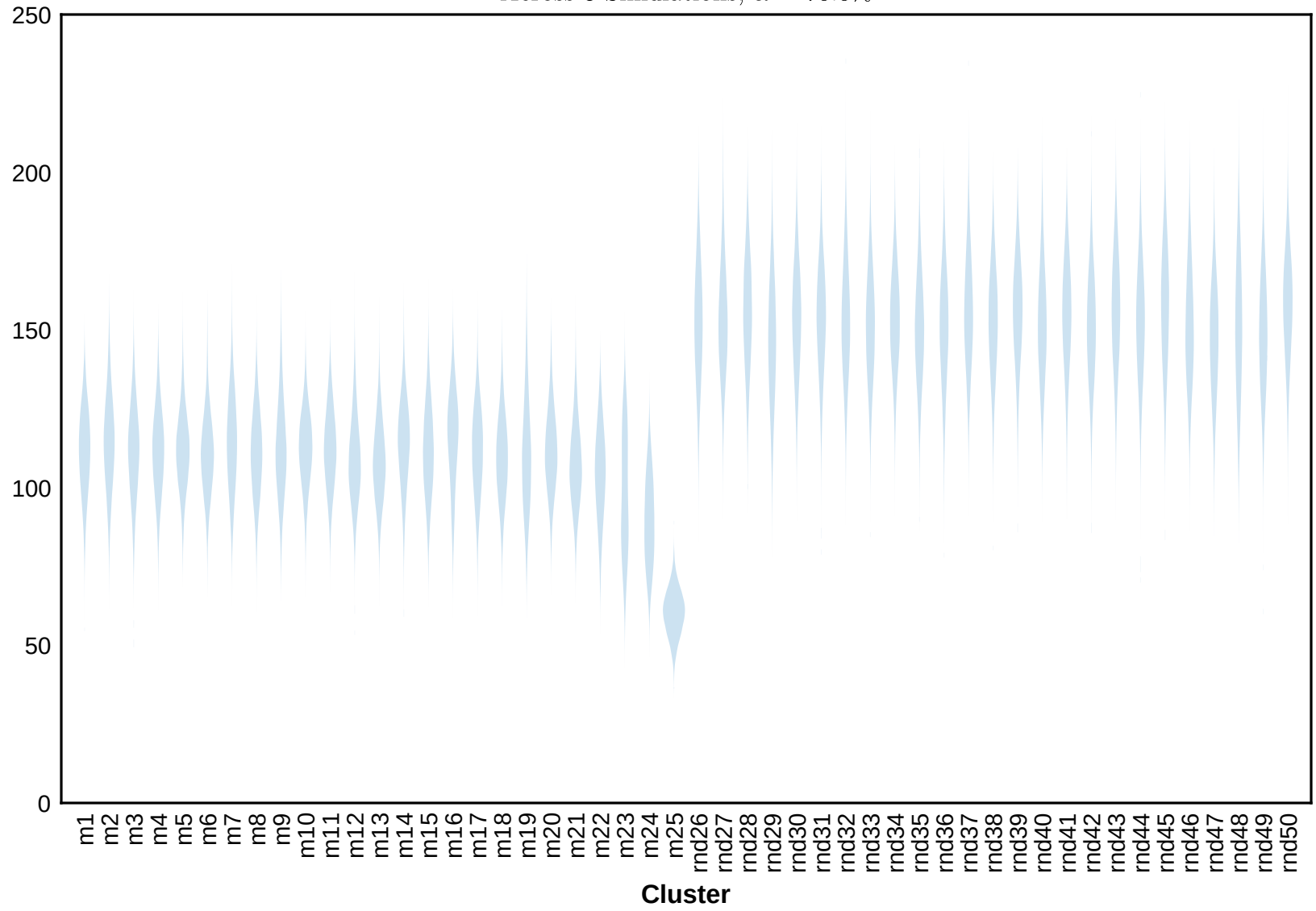
Aggregated Intra-cluster Distances Across 8 Simulations, \alpha = 70.0\%
