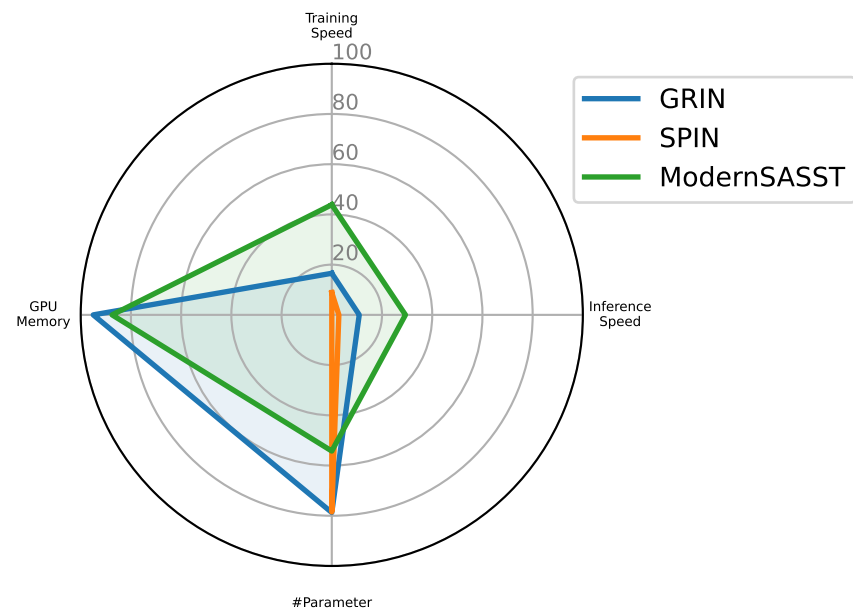
Imputation - AQI
