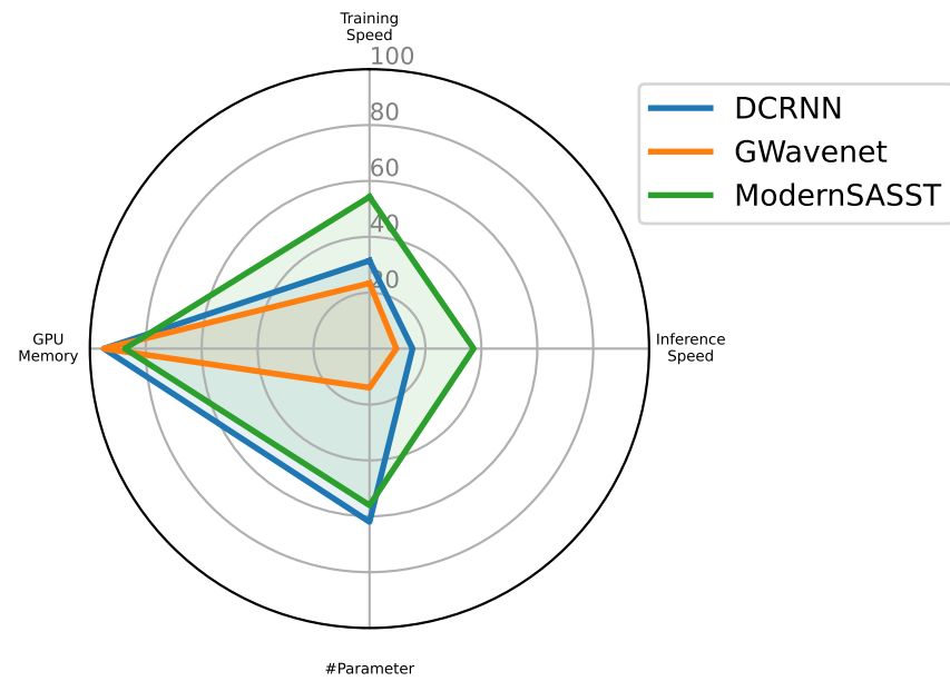
Forecasting - AQI
