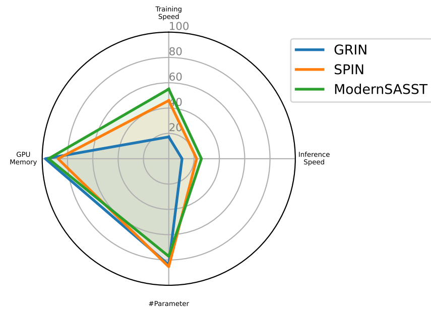
Imputation - SDWPF
