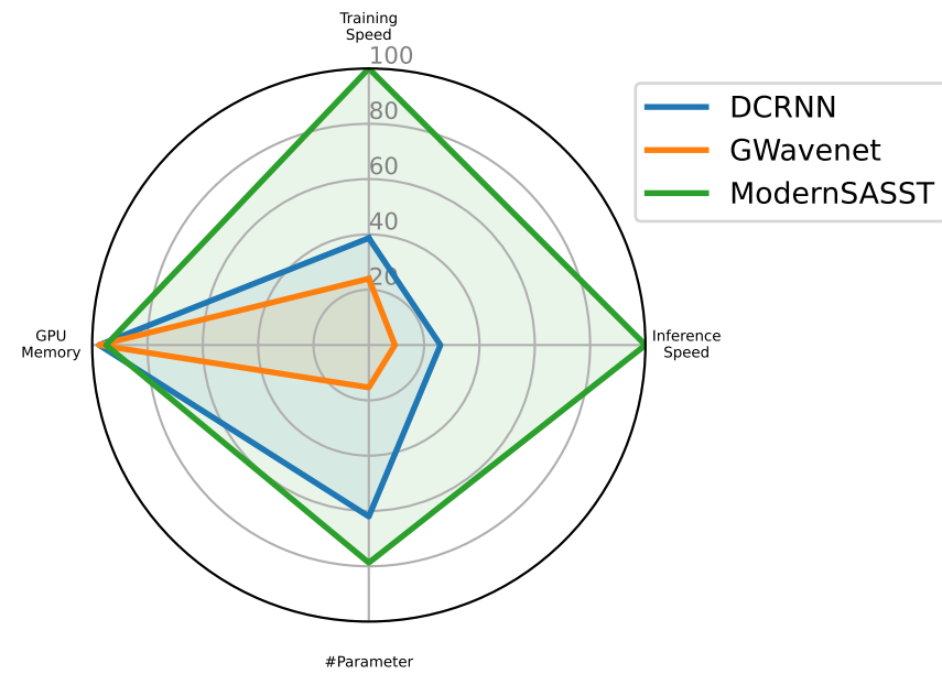
Forecasting - SDWPF
