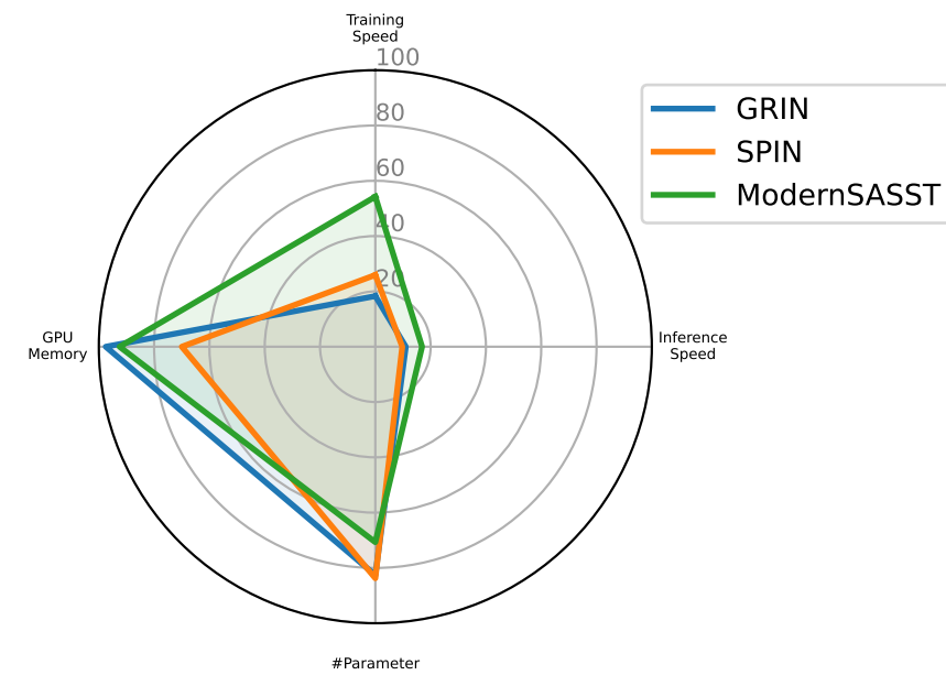
Imputation - MetrLA
