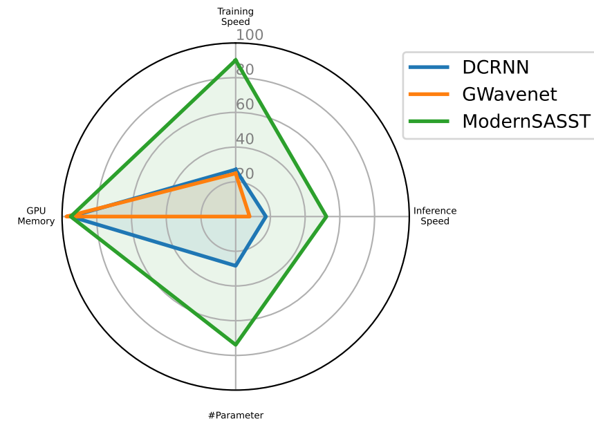
Forecasting - MetrLA
