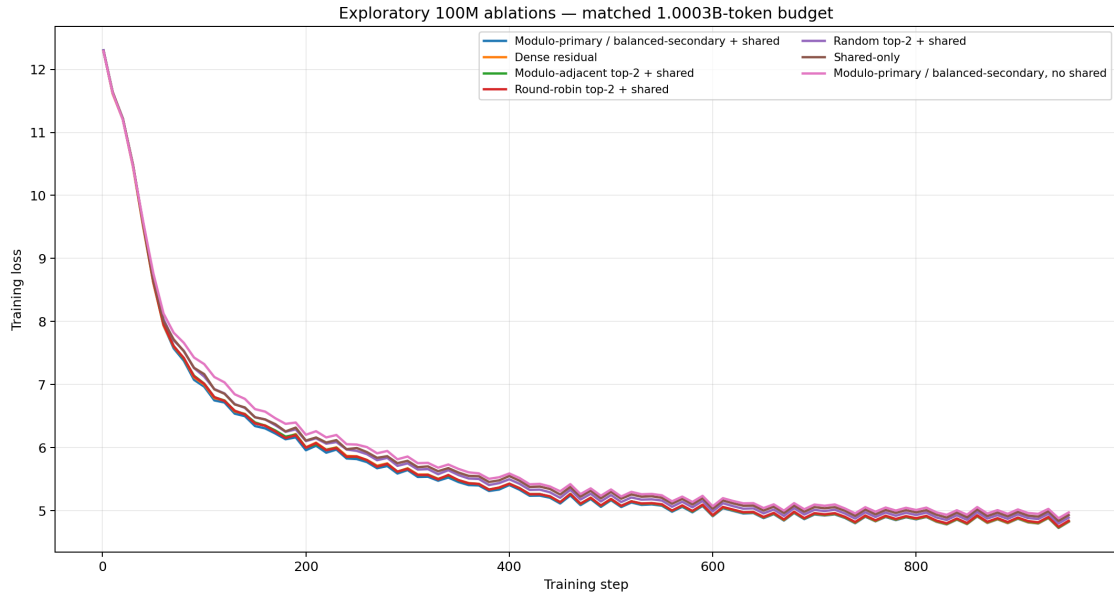
Figure 4: Exploratory 100M training curves at a matched 1.0003B-token budget. The condition originally logged as “Zipf shared” is identified by its realised fixed lookup: modulo-primary/balanced-secondary top-2. Single-run differences between modulo and round-robin controls are not interpreted causally.
