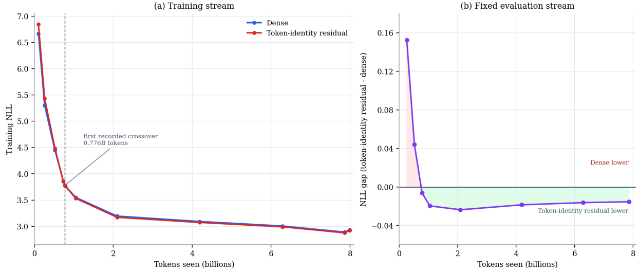
Figure 2: Matched-token loss measurements. Left: training NLL at recorded checkpoints. Right: token-identity residual minus dense NLL on the fixed FineWeb-Edu training-split evaluation stream; negative values favor the token-identity residual model. Markers are recorded checkpoints and lines guide the eye. The evaluation stream is not held out.
