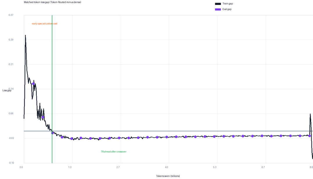
Figure 6: Training-loss gap at matched step (= matched tokens, iso-batch), computed as Token-Routed loss minus dense loss. Negative values indicate Token-Routed ahead. The gap is positive (TR behind) during the early specialization phase and first turns negative at the logged step 740.
