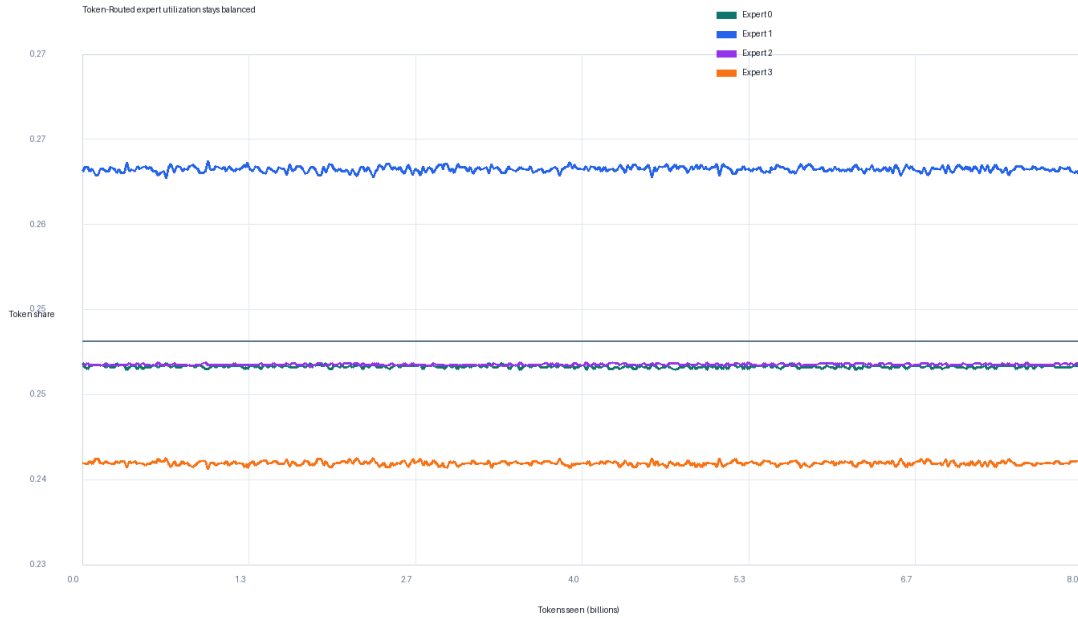
Figure 7: Expert utilization during the corrected 300M Token-Routed run. All four experts remain active and near-balanced; the observed matched-budget win is not caused by expert collapse.
