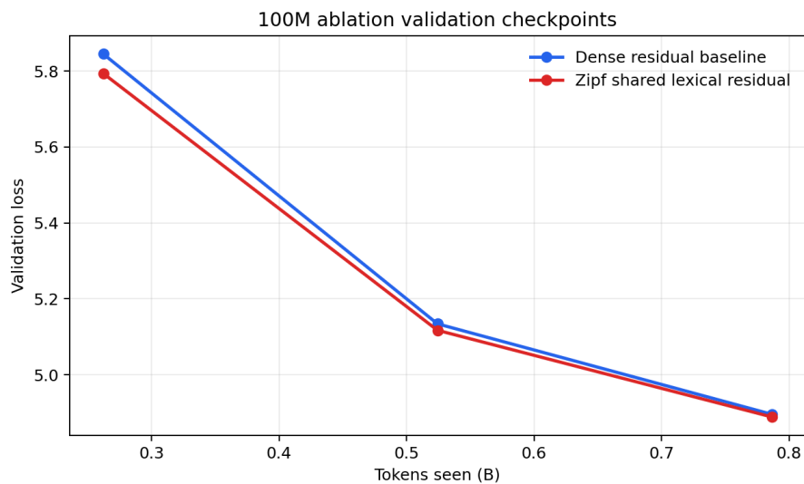
Figure 5: Validation checkpoints for the first two completed 100M ablation runs. Zipf shared reaches the lower validation loss at the best checkpoint observed so far (step 750).
