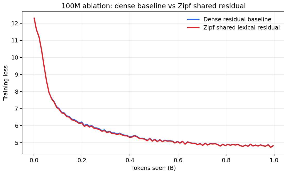
Figure 4: First completed 100M ablation curves on 2 \times B200 , matched at 1.0003B tokens. The Zipf shared lexical-residual variant finishes slightly ahead of the matched dense residual baseline on training loss.
