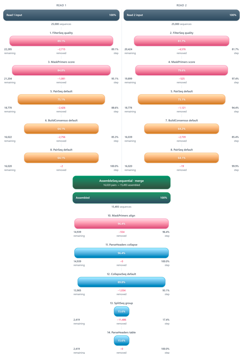
Figure S3: AIRRPrep read-retention visualization for the UMI-barcoded 5' RACE MiSeq 325+275 workflow of Supplementary Table S3 (SRR4026043, first 25,000 read pairs). Each box names its operation and shows the records entering and retained; R1 and R2 are counted separately until assembly, after which the merged stream is followed. The visualization can be exported as a PNG.
