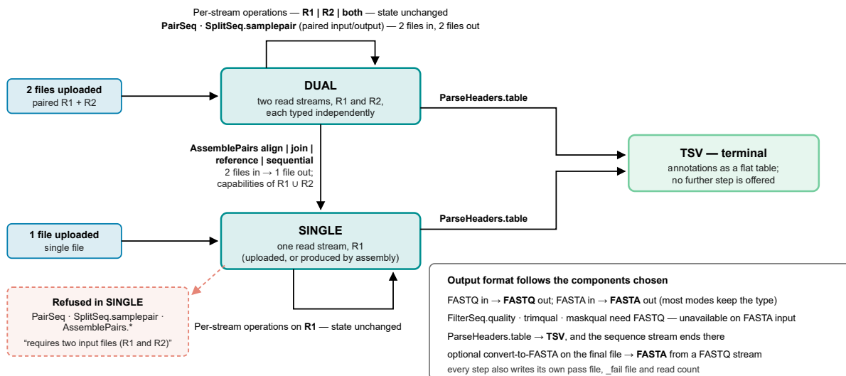
Figure S4: Read-stream behaviour of bulk operations. An operation may act on the Read 1 (R1) or Read 2 (R2) stream independently, require both streams and keep them separate (for example PairSeq.py ), or merge the two streams into a single sequence stream ( AssemblePairs.py ). Read streams are called R1 and R2 throughout this work, never “lane”: a sequencing flow-cell lane is a different thing and is not referred to anywhere here. The four assembly operations, written AssemblePairs.py align , join , reference and sequential in this supplement and in every table, are the components the interface labels AssembleSeq.align , AssembleSeq.join , AssembleSeq.reference and AssembleSeq.sequential ; that family is the only name that differs between the interface and pRESTO (Supplementary Table S2).
