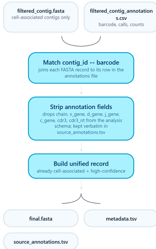
Figure S1: Representative AIRRPrep single-cell workflow visualization for a Cell Ranger V(D)J filtered contigs input. The application displays the processing route associated with the selected single-cell input and allows the workflow graphic to be exported as a PNG; this figure is that export. The annotation fields the Strip annotation fields step removes from the normalized record are not discarded, which is why the run writes three files: they are kept unchanged in source_annotations.tsv , keyed on the same sequence_id as final.fasta and metadata.tsv (Supplementary Table S1).
