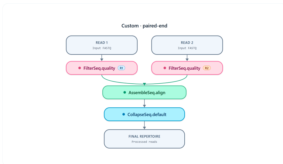
Figure S2: Representative AIRRPrep paired-read bulk workflow visualization. Read 1 (R1) and Read 2 (R2) are shown through the operations applied to each read stream and, where applicable, their transition to a merged sequence stream after assembly. The workflow graphic can be exported from AIRRPrep as a PNG.
