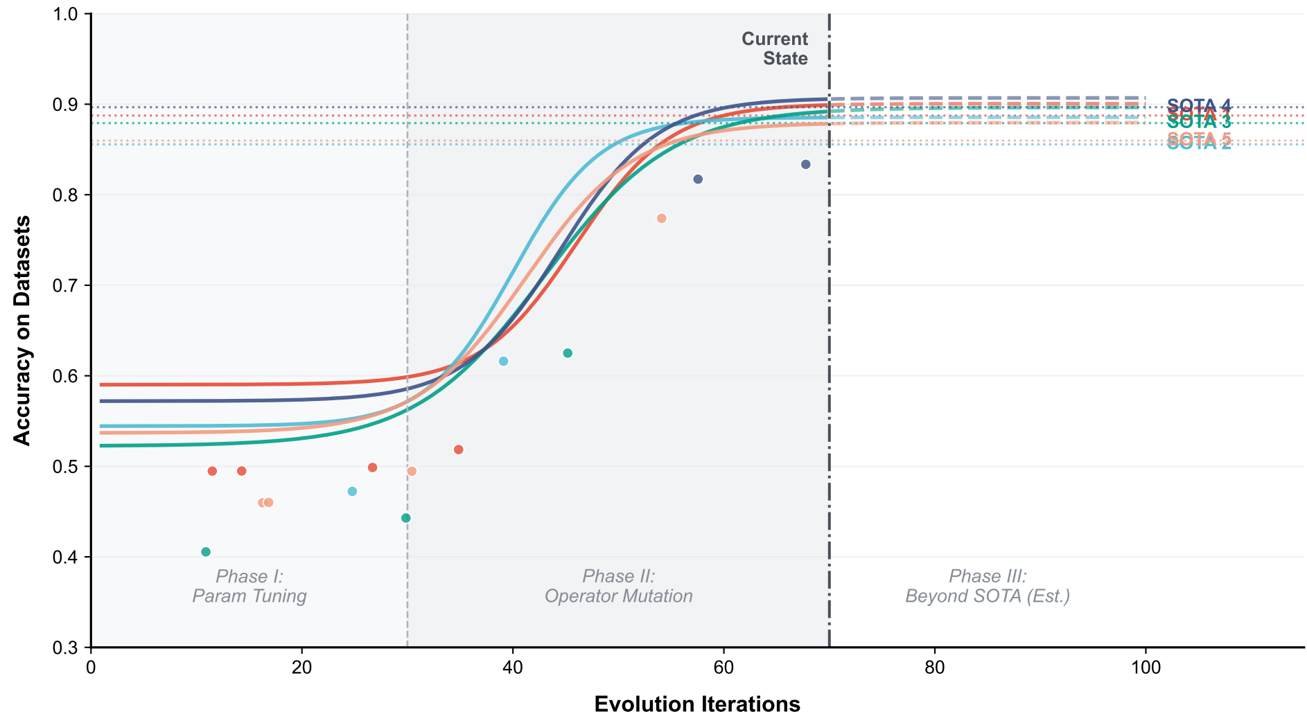
Performance Trajectory of Auto-Evolved Feature Selection Operators
