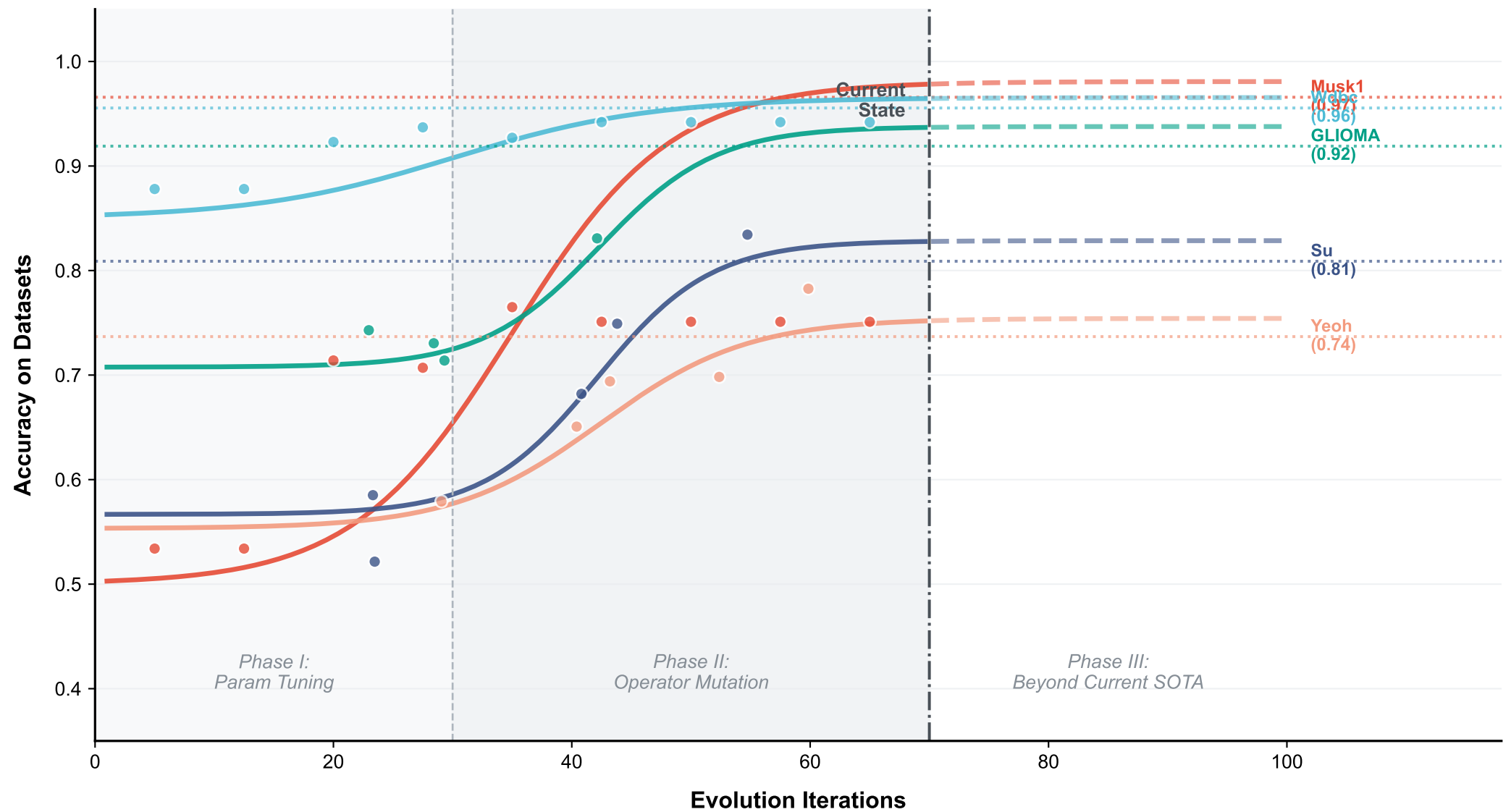
Performance Trajectory of Evolved Feature Selection Operators
