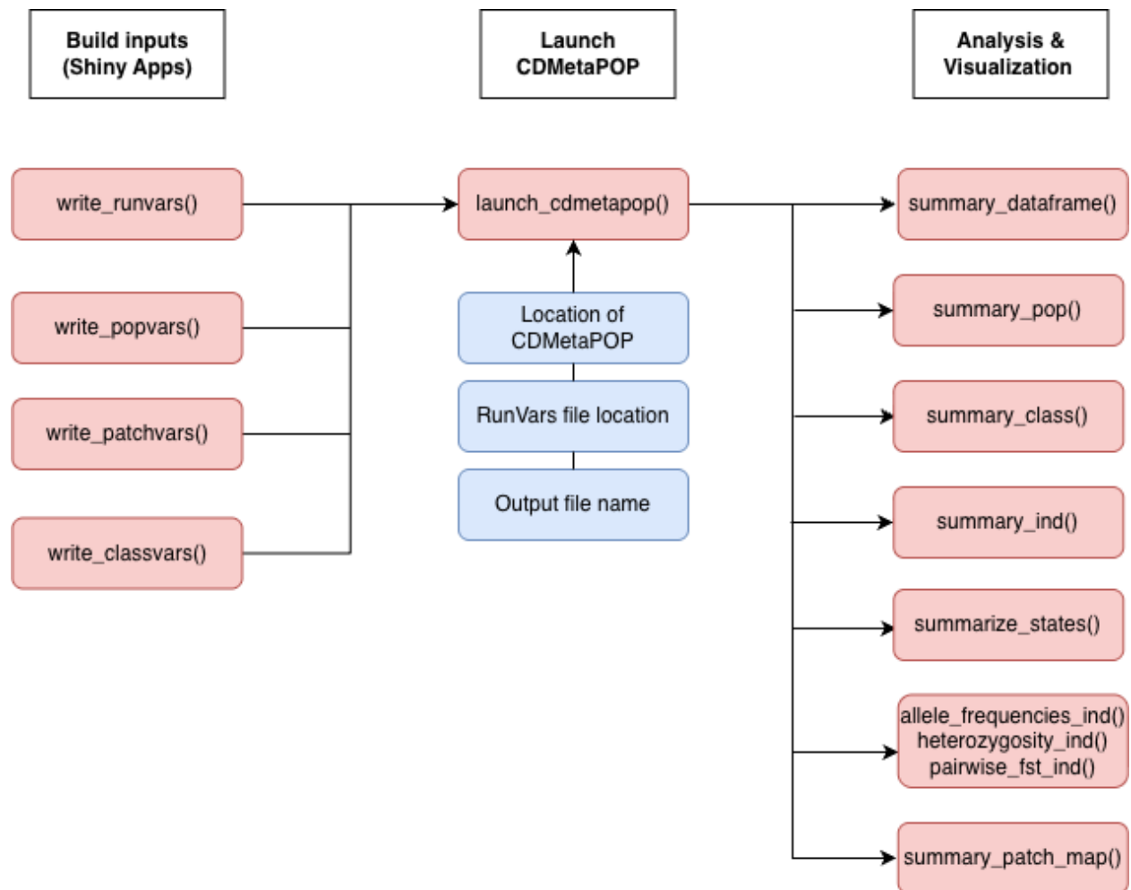
Figure 1: Figure 1: cdmetapop.R package structure.
