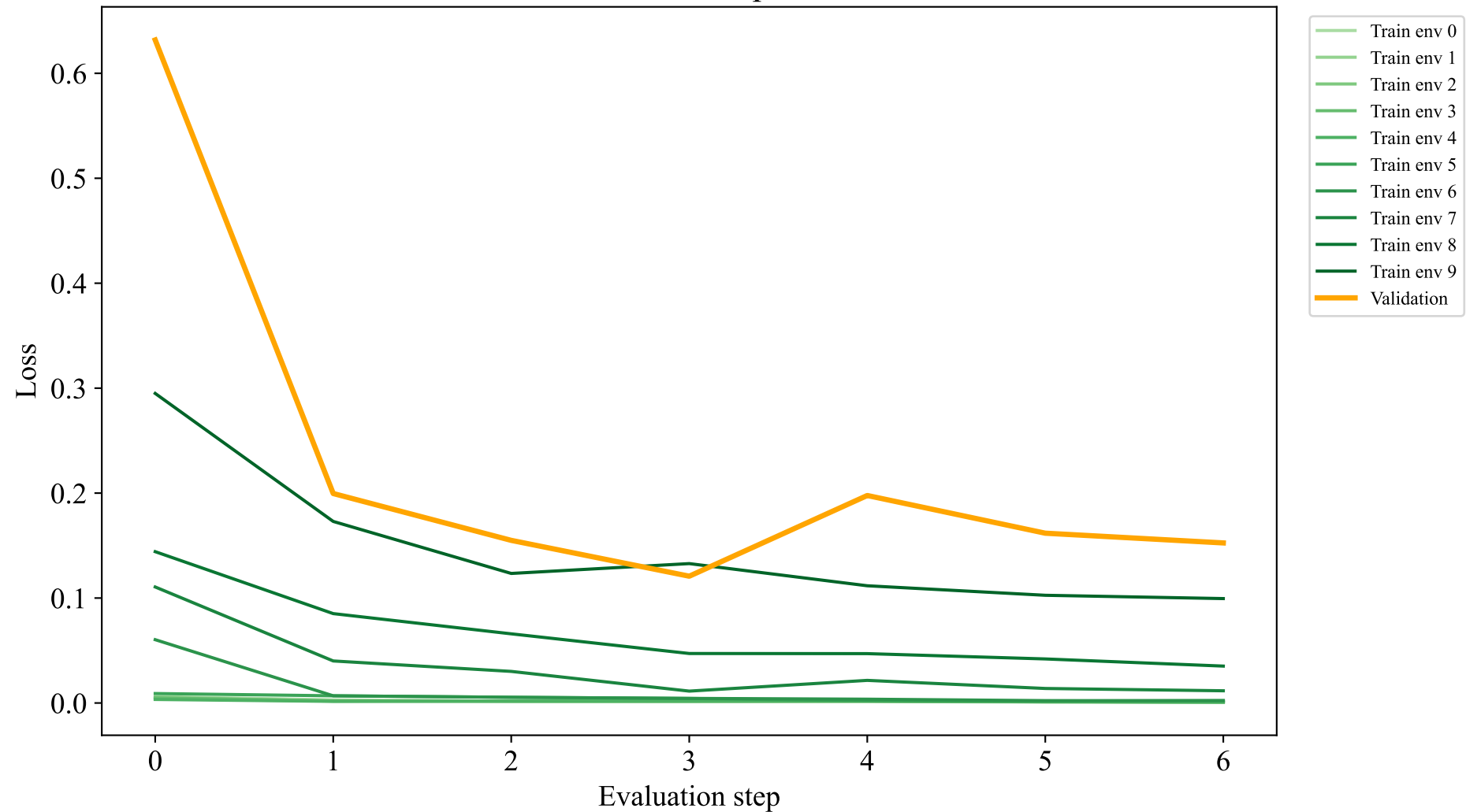
Train and validation loss per environment
