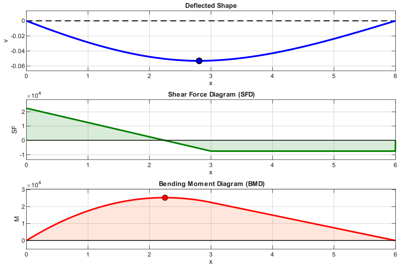
Nodal Deflections
