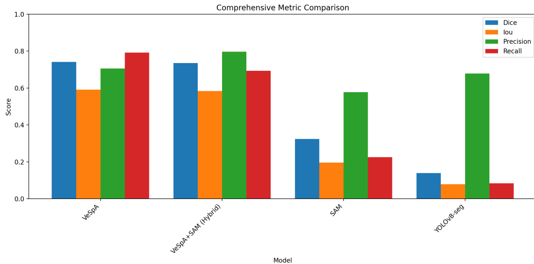
Figure 4: Comprehensive comparison of Dice, IoU, precision, and recall across the four evaluated segmentation methods.
