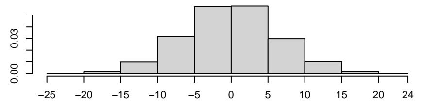
Density of nodematch.grade
