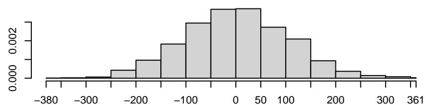
Density of nodeocov.grade
