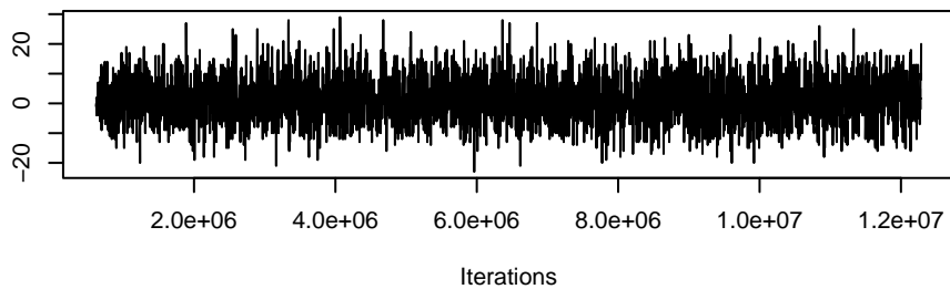
Trace of nodeifactor.gender_recode.male
