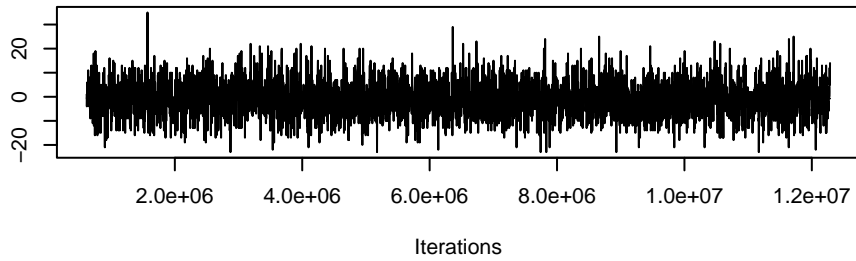
Trace of nodematch.gender_recode
