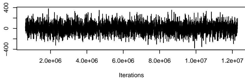
Trace of nodeicov.grade
