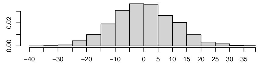
Density of edges
