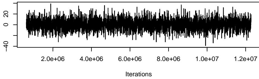
Trace of edges
