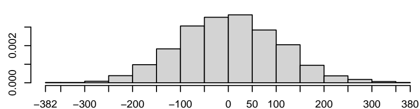
Density of nodeicov.grade
