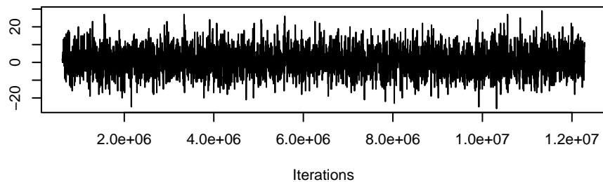
Trace of nodeofactor.gender_recode.male
