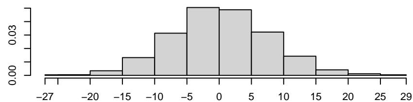
Density of nodeofactor.gender_recode.male
