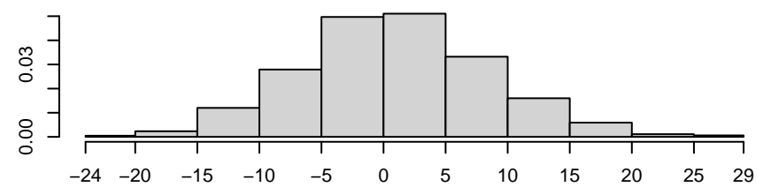
Density of nodeifactor.gender_recode.male
