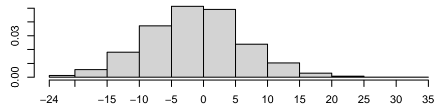
Density of nodematch.gender_recode
