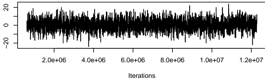
Trace of nodematch.grade
