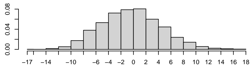
Density of mutual
