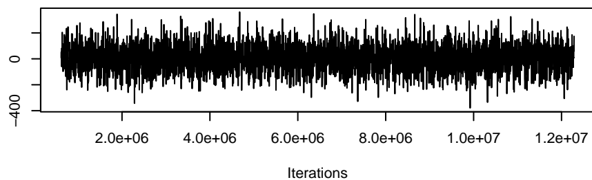
Trace of nodeocov.grade
