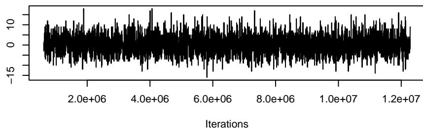
Trace of mutual
