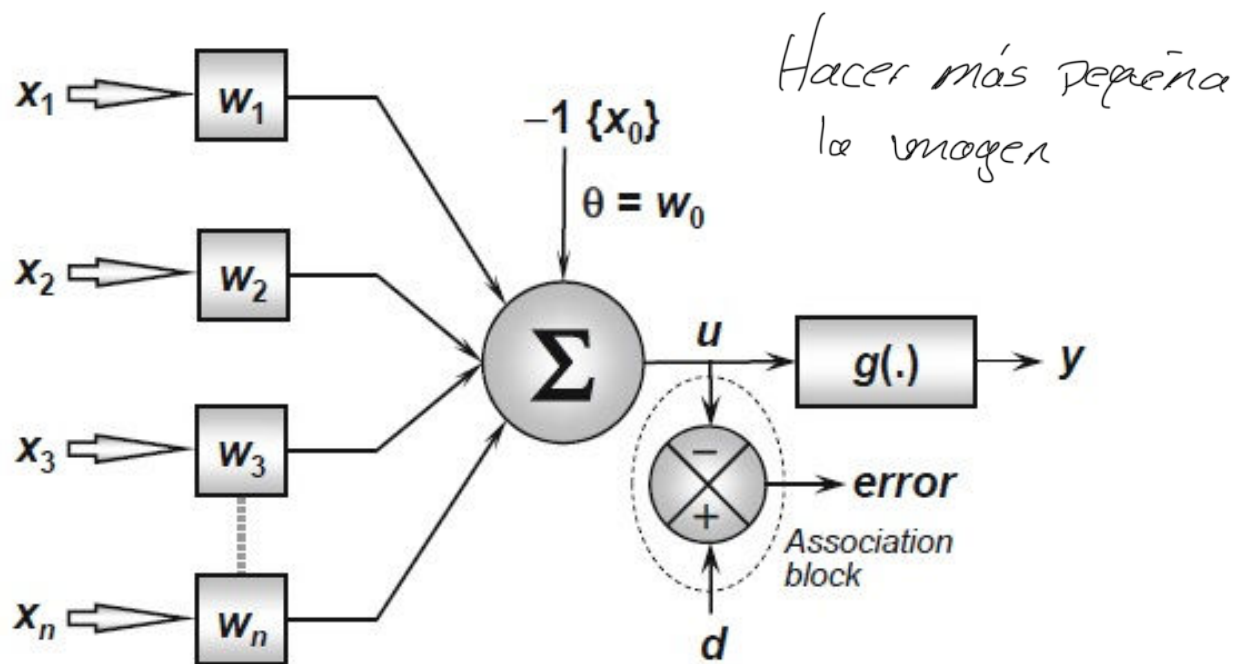
Figura 2: Red Neuronal Artificial Básica
