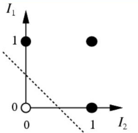
Figure 4: OR logic gate in the input plane.
