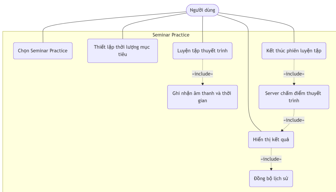
Figure 7: Objective 2 Use Case Diagram
