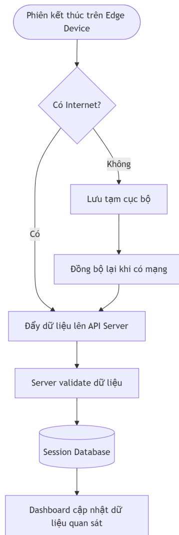
Figure 17: Synchronization Flow Diagram
