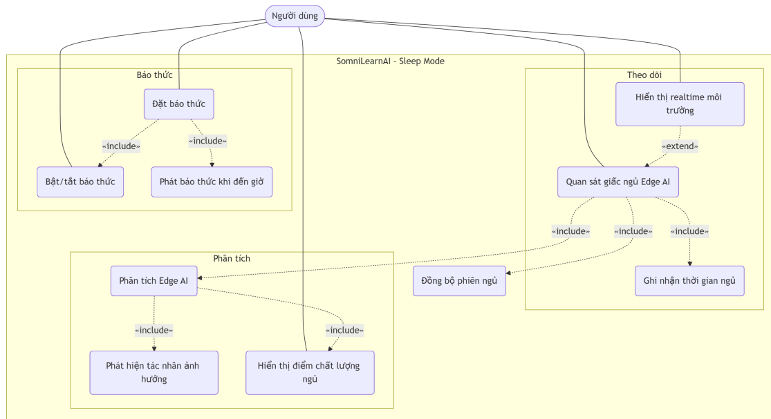
Figure 8: Sleep Monitoring Edge AI Use Case Diagram
