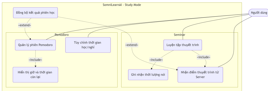
Figure 5: Pomodoro Timer Use Case Diagram
