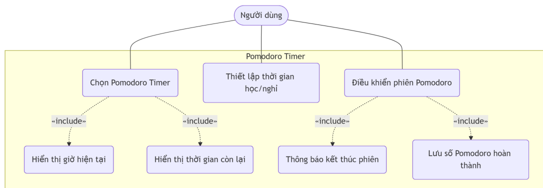
Figure 6: Pomodoro Timer Use Case Diagram
