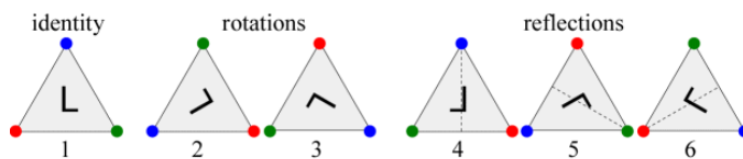
Figure 1: Elements of the Dihedral Group D_3
