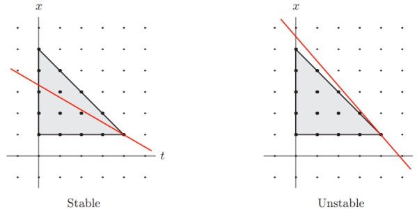
Figure 7: Geometric intuition for the CFL condition
