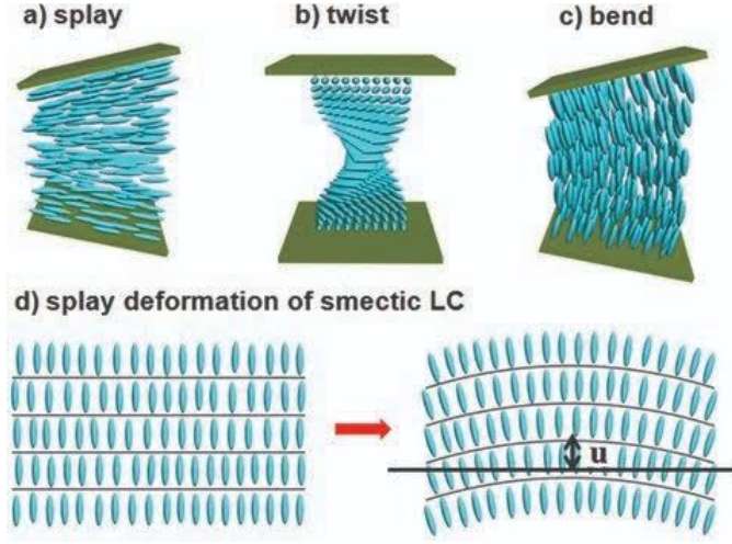
Figure 4: The three different types of deformations in liquid crystals. Notice the difference in the director axis between bending and splaying.
