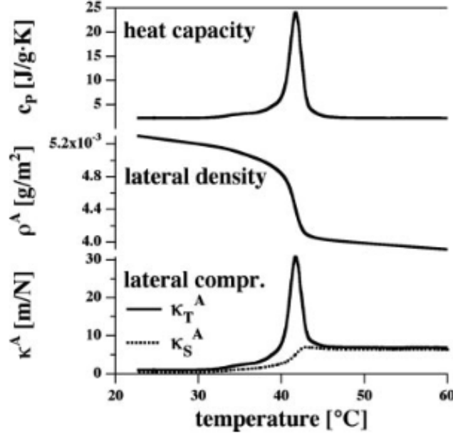
Figure 2: Data from Heimburg and Jackson describing the heat capacity of DPPC large unilamellar vesicle (Top), lateral area density, \rho^A (Middle), and the corresponding lateral compressibility (Bottom) (isothermal area compressibility, solid curve, corresponding to a low-frequency case and adiabatic area compressibility, dotted line, corresponding to a 5-MHz ultrasonic experiment), as calculated from the heat capacity.
