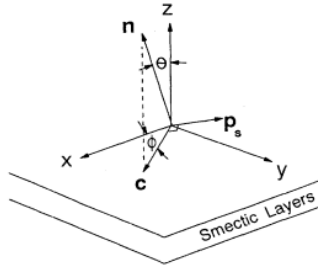
FIG. 1. Sketch of the ferroelectric liquid crystal geometry. The smectic-C* phase has layering along the z direction. The molecular director \mathbf{n} is tilted from the layer normal by an angle \theta and the spontaneous polarization \mathbf{p}_s is along the direction defined by \mathbf{i}_z \times \mathbf{n} . \mathbf{c} represents the c director, which lies in the smectic plane and is perpendicular to \mathbf{p}_s .
