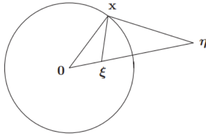
Figure 1: Method of Images for a singular charge in a unit disk
