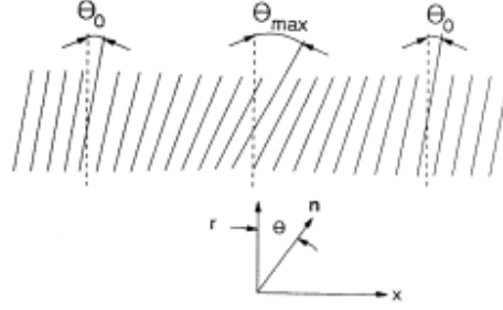
FIG. 3. Splay wave in a 1D membrane. \theta_0 is the equilibrium-tilt angle of the local molecular director with respect to the layer normal, i.e., the r direction. \theta_{max} is the maximum tilt at the peak of the splay wave.
