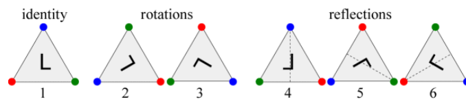
Figure 1: Elements of the Dihedral Group D_3
