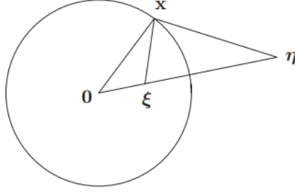
Figure 1: Method of Images for a singular charge in a unit disk
