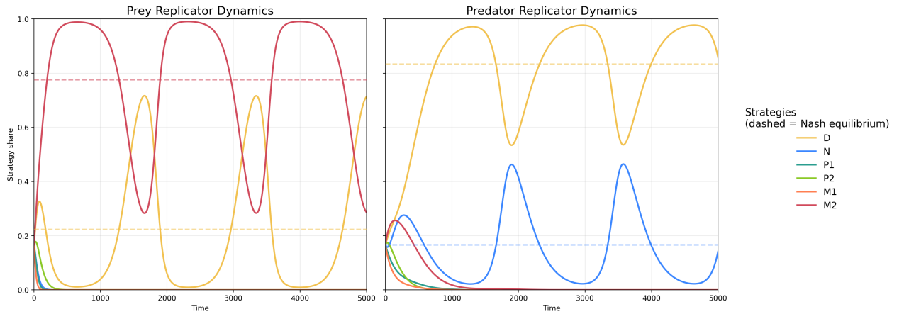
Figure 10: Representative asymmetric replicator dynamics for the balanced case (w_1, w_2) = (0.5, 0.5) , initialized from the uniform strategy distribution. The left panel shows prey strategy frequencies and the right panel shows predator strategy frequencies. The dominant strategies remain concentrated on the support highlighted by the mixed Nash equilibrium, but the trajectory exhibits persistent oscillations rather than monotone convergence to a fixed point.
