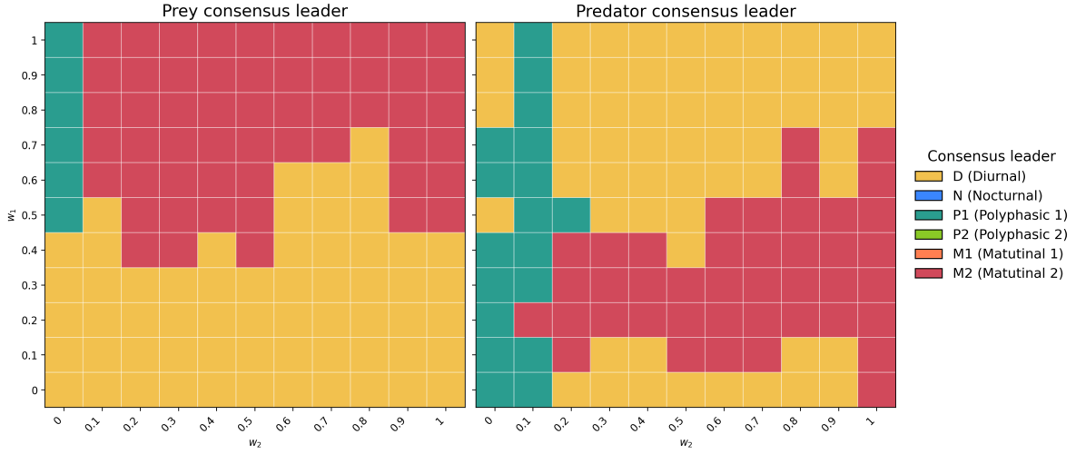
Figure 9: Consensus leading component of the mixed Nash equilibrium as a function of the prey sight weight w_1 and predator sight weight w_2 . Each cell corresponds to one weight pair and is labeled by the strategy with the largest probability in the unique mixed Nash equilibrium. The left panel shows the prey leader and the right panel shows the predator leader.
